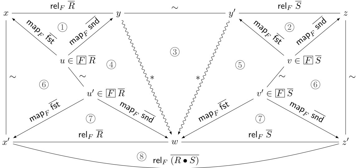
Figure 1: Proof diagram for Theorem 3.21
